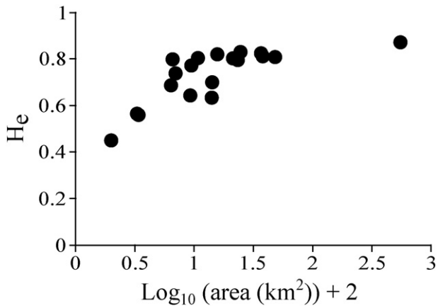
Fig. 2. Relationship between lake surface area in km 2 , given as \log_{10}(\text{area}) + 2 , and expected heterozygosity calculated from stickleback microsatellite data.
